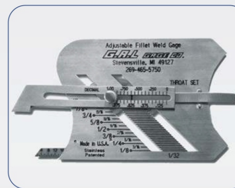
ADJUSTABLE FILLET WELD GAUGE
