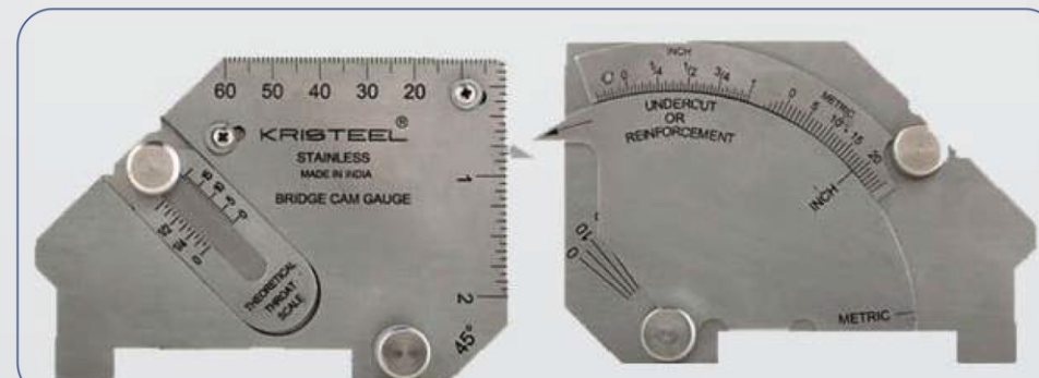
UNIVERSAL WELDING GAUGE
